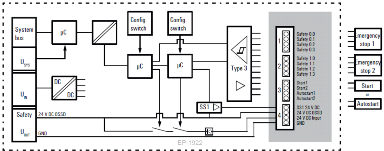
Block Diagram EP-1922
