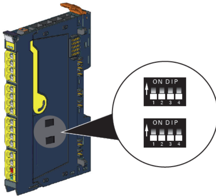
DIP Switch on the EP-1922
